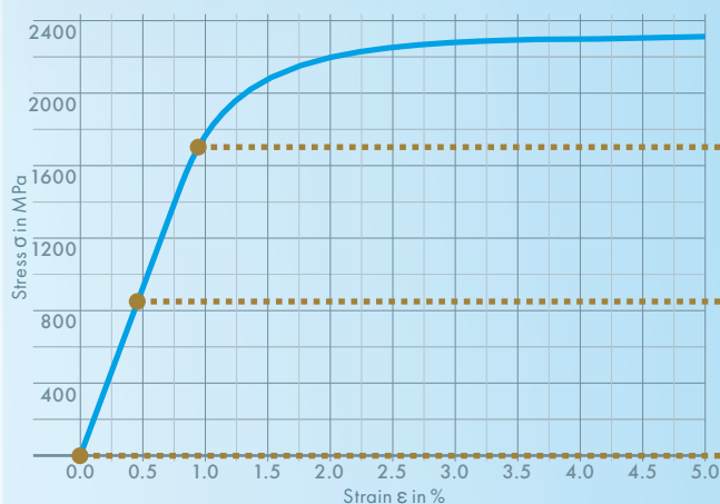
应变应力图 - 不锈钢圆钢丝 d = 1.9 mm - RM = 2300 MPa
